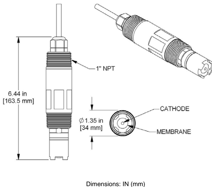
Dimensions: IN (mm) Figure 3.2: 1 Inch Sensor Body
